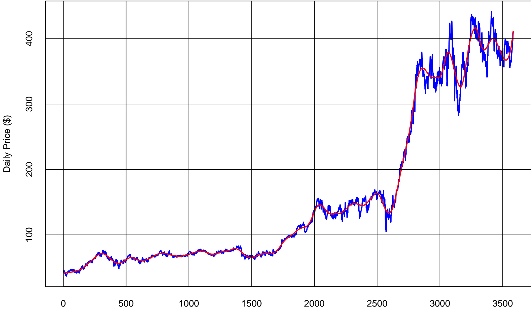
Trading Days Jan 1 2010 to Present Price (Blue) Smoothed Trend (Red)
